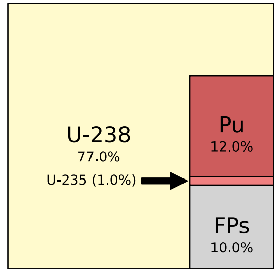
Typical breeder (first cycle)
